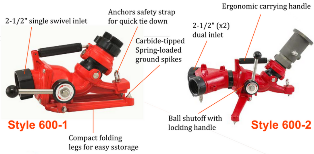
600-1 Single-Inlet Portable Ground Monitor 600-2 Dual-Inlet Portable Ground Monitor
